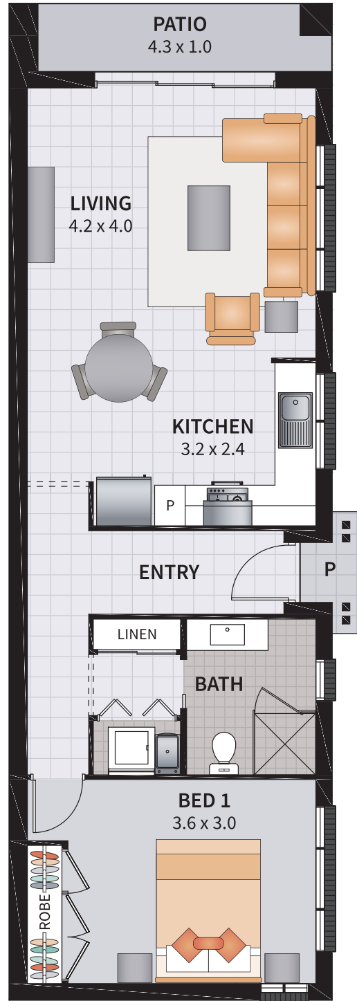
GRANNY FLAT OPTION 2 1 BEDROOM / ALTERNATE BATH
